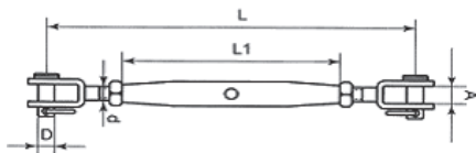
Syrefast, AISI 316 Vantskrue, AISI 316, Gaffel/Gaffel S.S., AISI 316 Closed Body Rigging Screw, Jaw/Jaw
